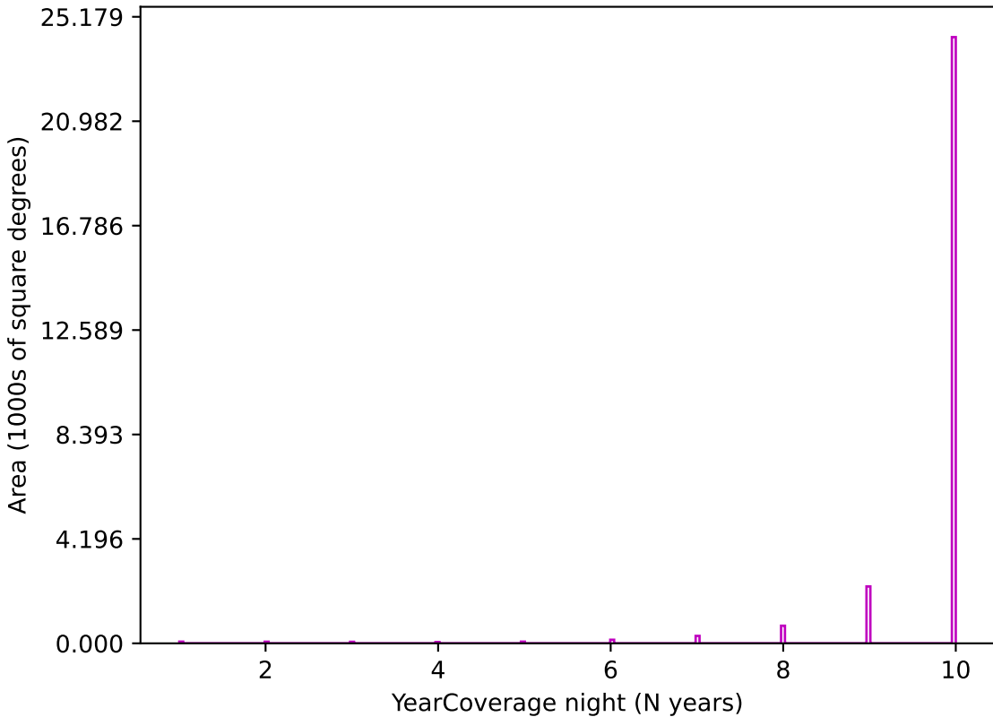
too_10_4v3.4_10yrs z band: YearCoverage night
