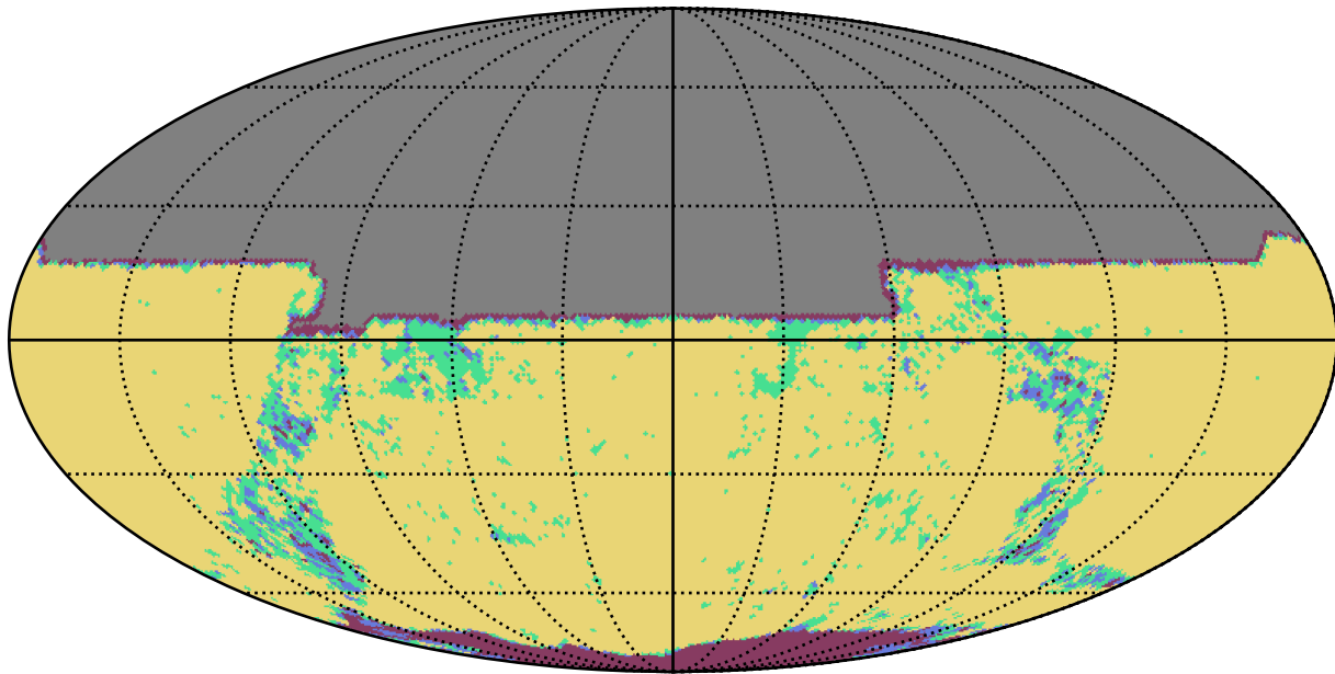
too_10_4v3.4_10yrs y band: YearCoverage night
