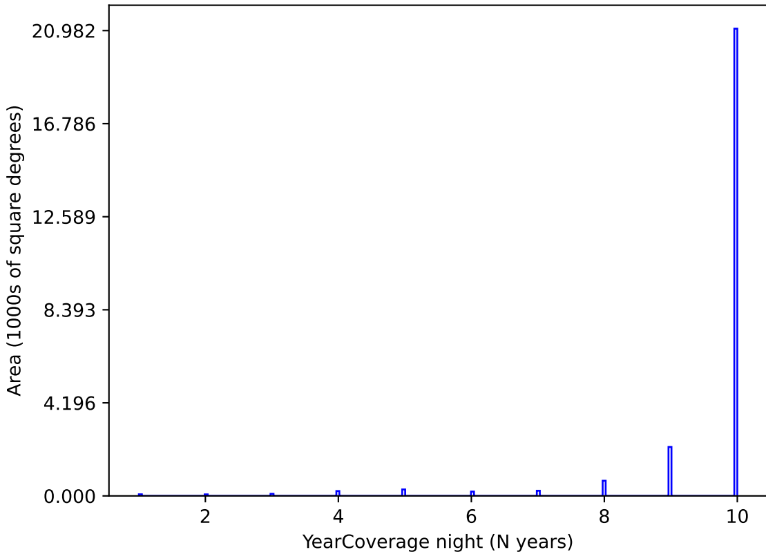
too_10_4v3.4_10yrs y band: YearCoverage night
