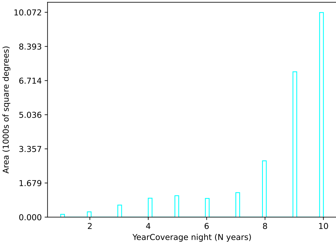
too_10_4v3.4_10yrs u band: YearCoverage night
