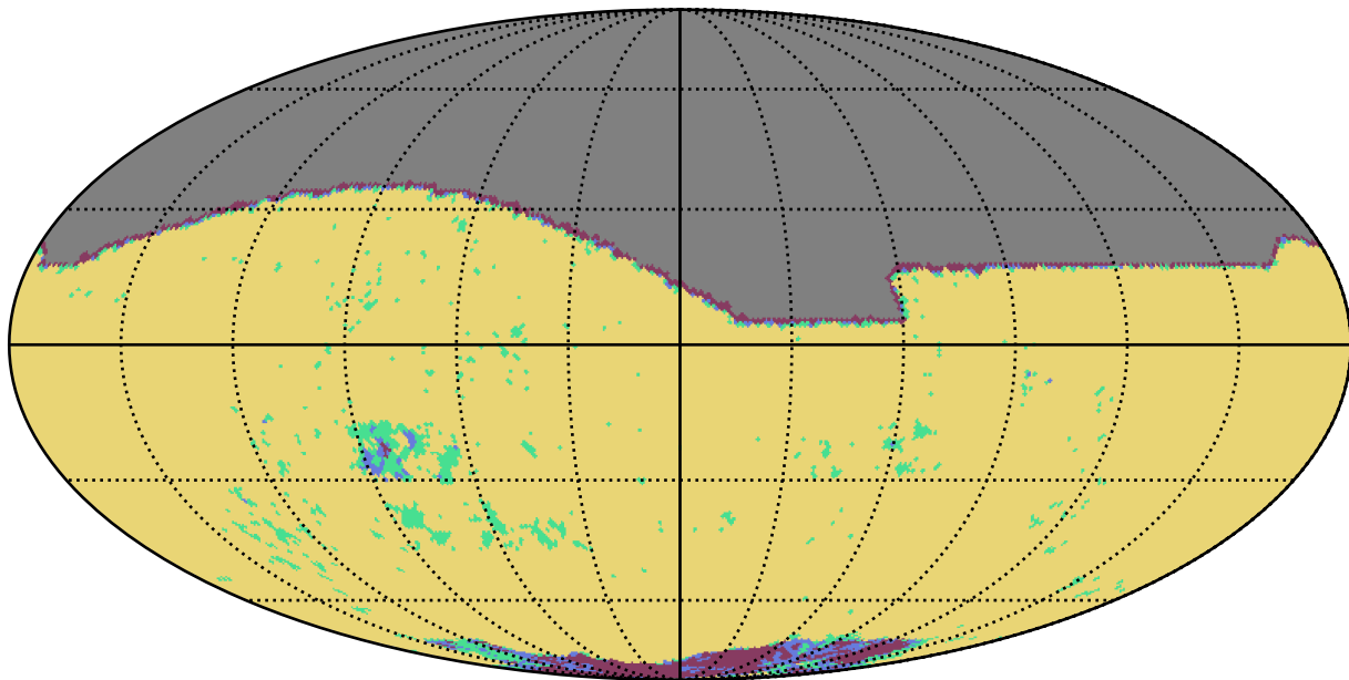
too_10_4v3.4_10yrs r band: YearCoverage night
