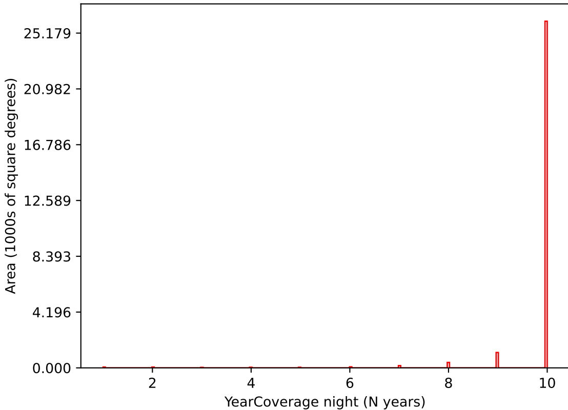
too_10_4v3.4_10yrs i band: YearCoverage night
