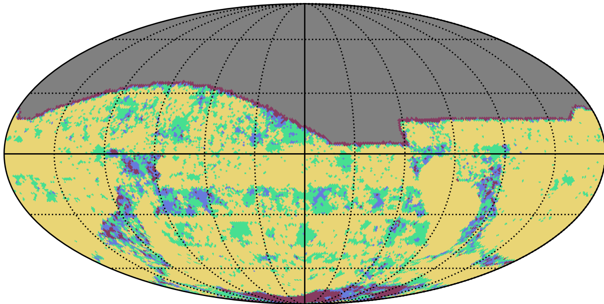
too_10_4v3.4_10yrs g band: YearCoverage night
