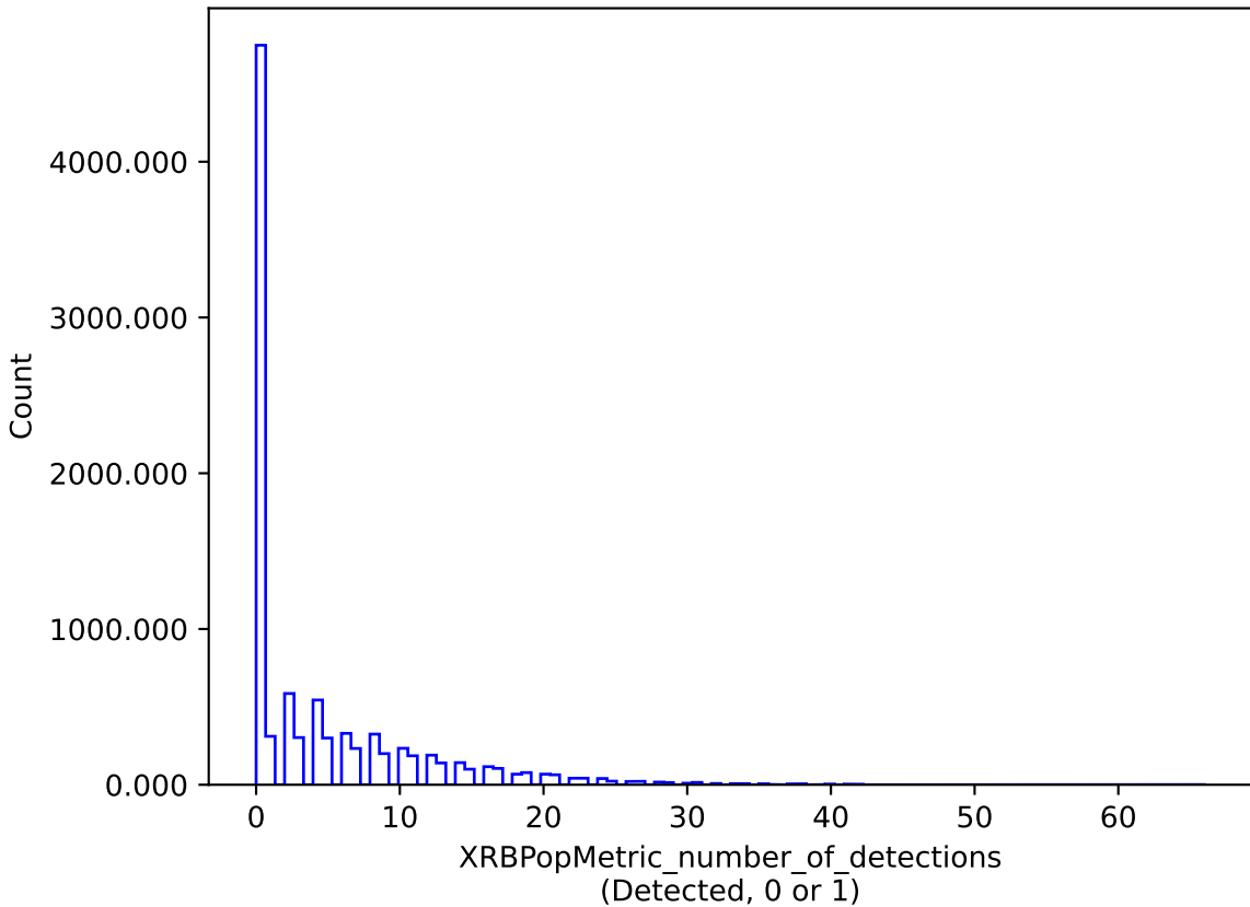
too_10_4v3.4_10yrs : XRBPoMetric_number_of_detections
