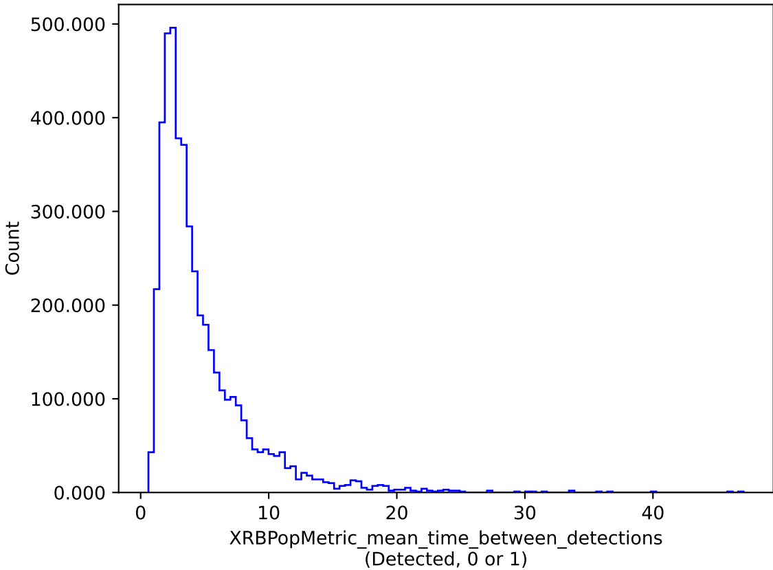
too_10_4v3.4_10yrs : XRBPoMetric_mean_time_between_detections
