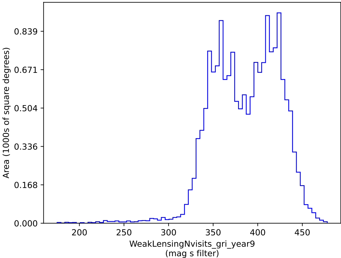
too_10_4v3.4_10yrs gri band non-DD: WeakLensingNvisits_gri_year9
