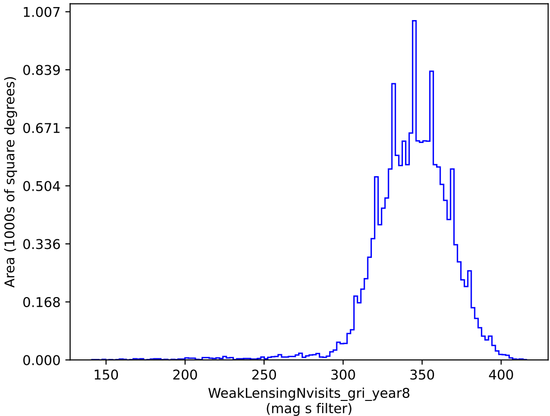
too_10_4v3.4_10yrs gri band non-DD: WeakLensingNvisits_gri_year8
