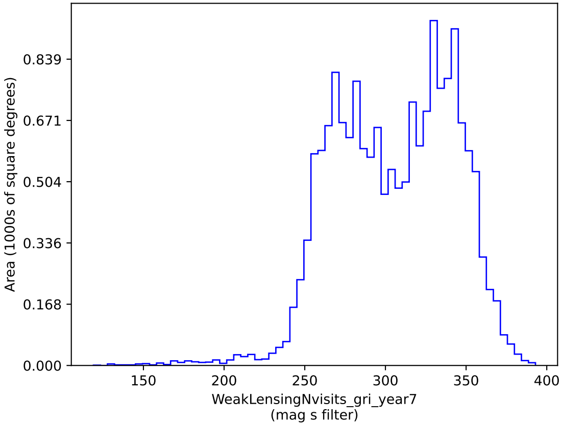
too_10_4v3.4_10yrs gri band non-DD: WeakLensingNvisits_gri_year7
