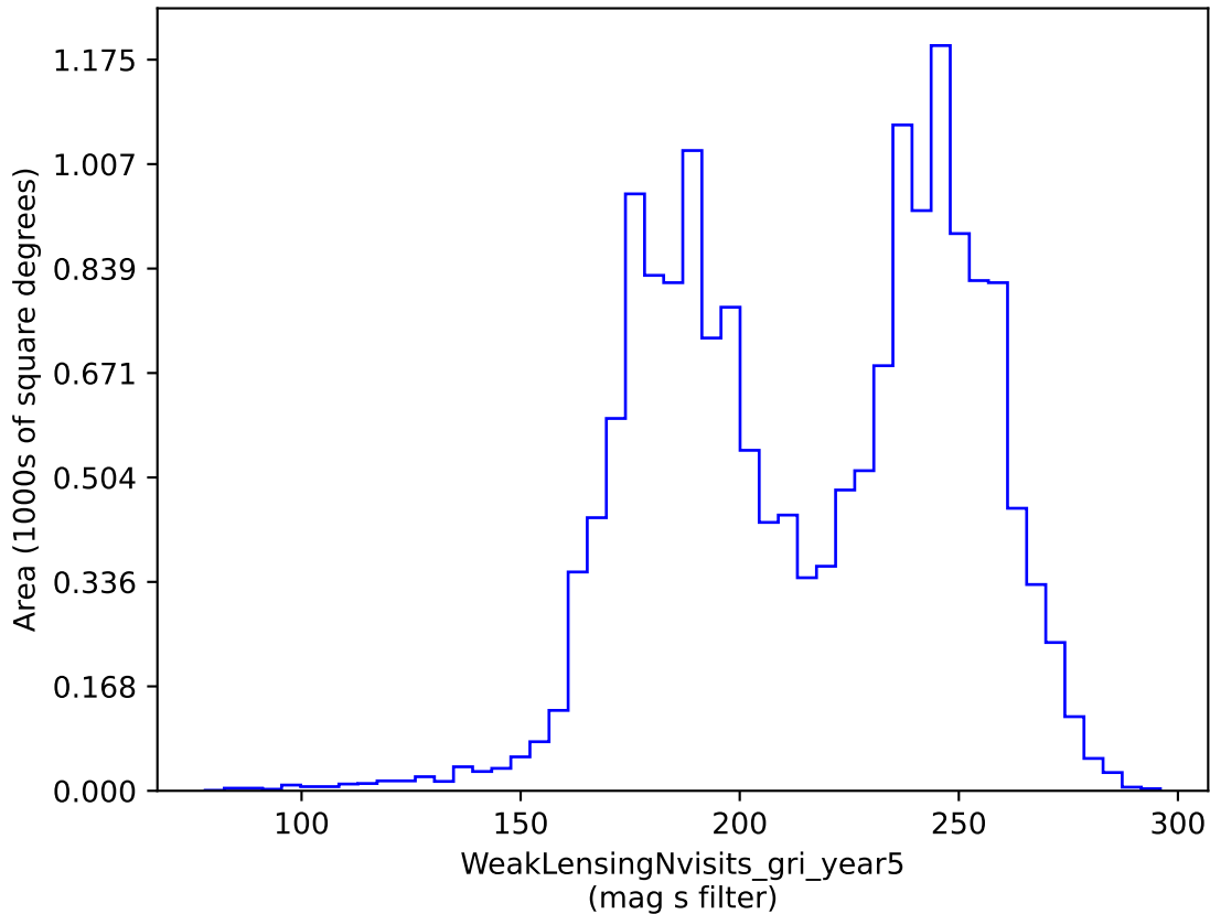
too_10_4v3.4_10yrs gri band non-DD: WeakLensingNvisits_gri_year5
