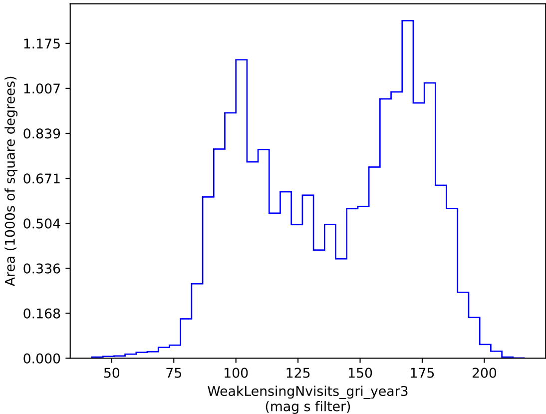
too_10_4v3.4_10yrs gri band non-DD: WeakLensingNvisits_gri_year3
