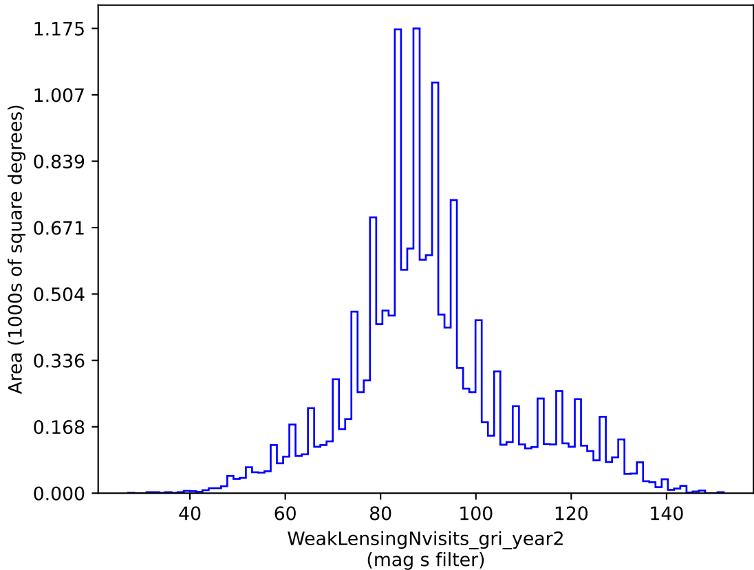
too_10_4v3.4_10yrs gri band non-DD: WeakLensingNvisits_gri_year2
