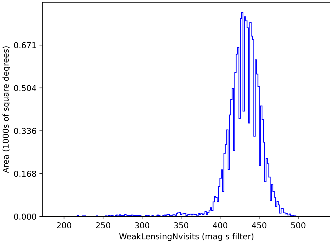
too_10_4v3.4_10yrs gri band non-DD: WeakLensingNvisits
