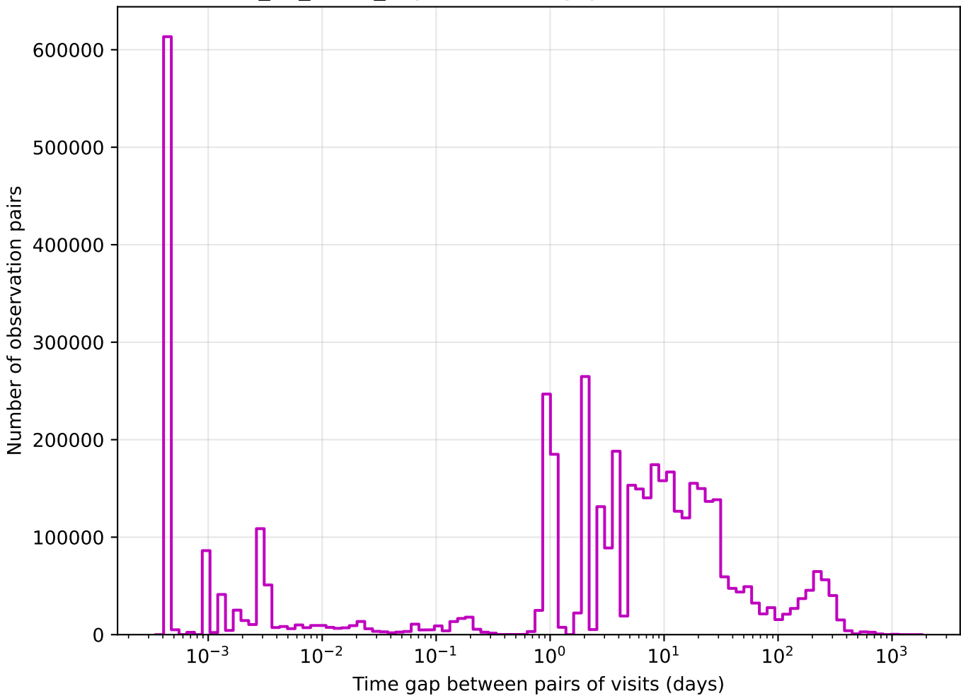
too_10_4v3.4_10yrs z band: Tgaps observationStartMJD
