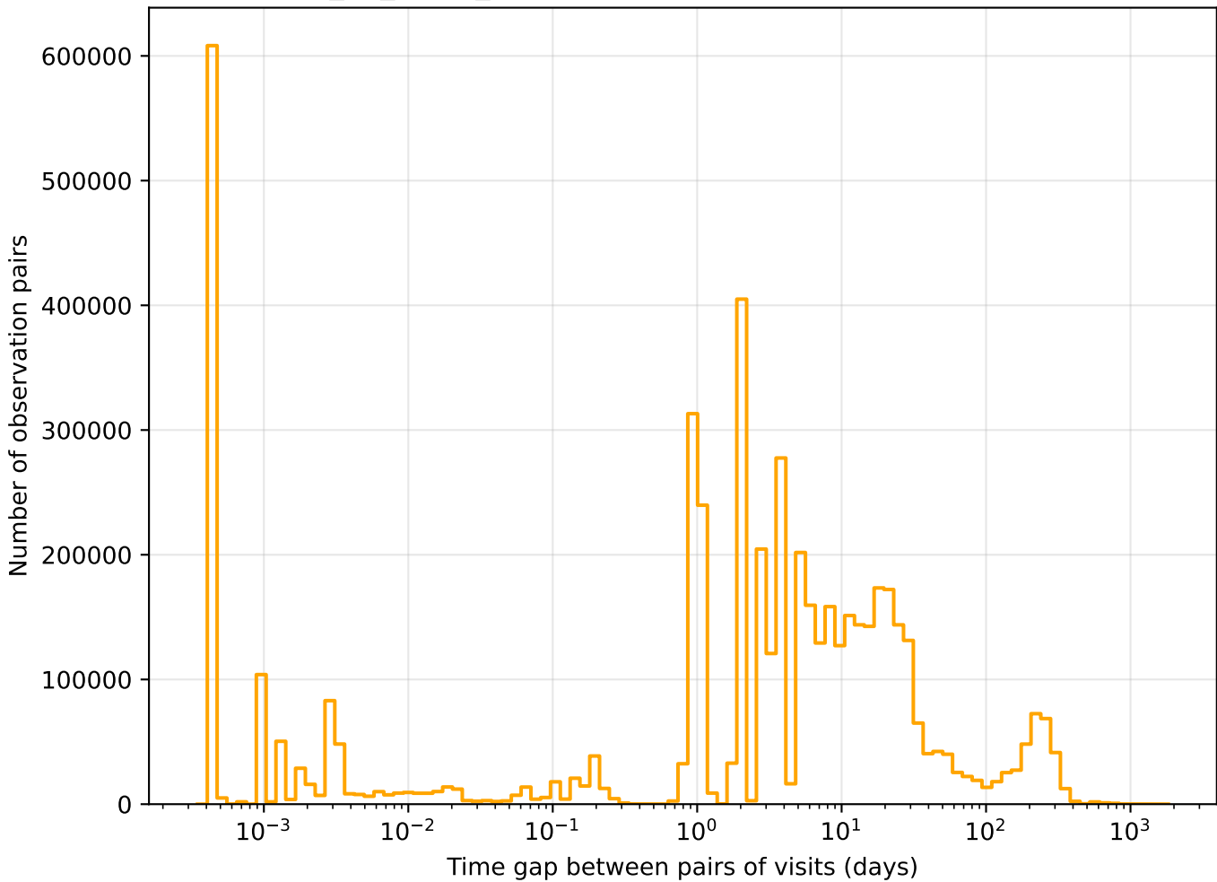
too_10_4v3.4_10yrs r band: Tgaps observationStartMJD
