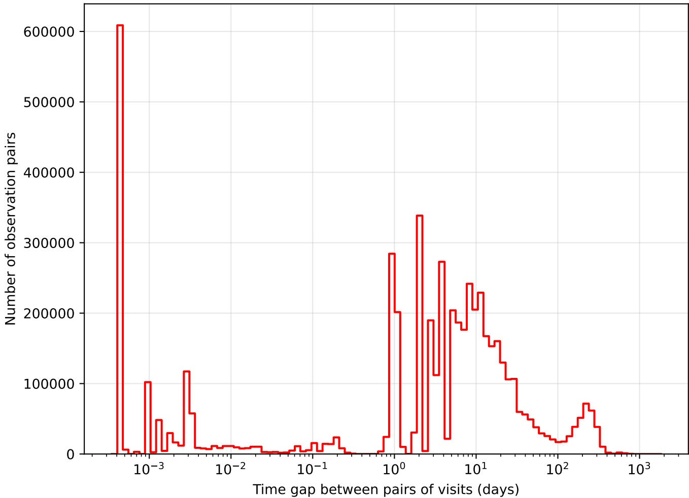
too_10_4v3.4_10yrs i band: Tgaps observationStartMJD
