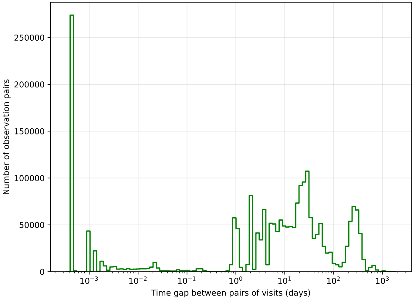
too_10_4v3.4_10yrs g band: Tgaps observationStartMJD
