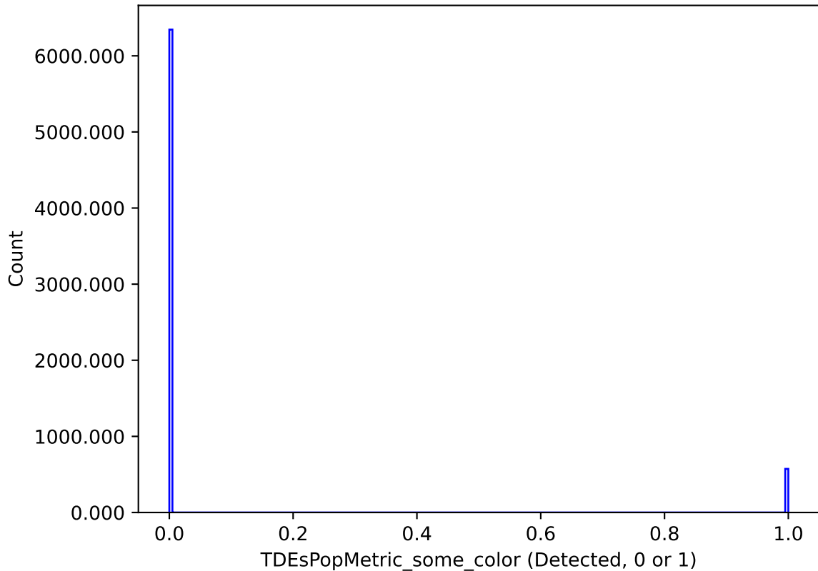
too_10_4v3.4_10yrs : TDEsPopMetric_some_color
