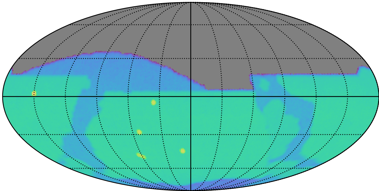
too_10_4v3.4_10yrs z: SurfaceBrightLimit
