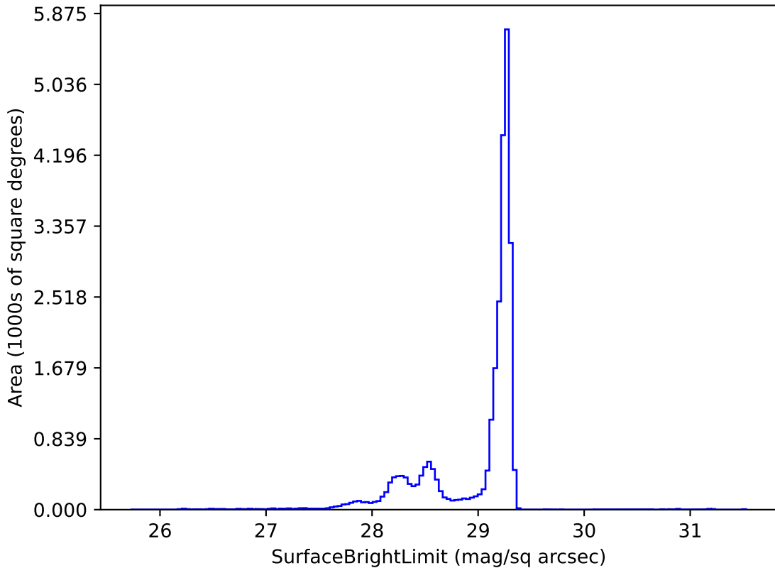
too_10_4v3.4_10yrs z: SurfaceBrightLimit
