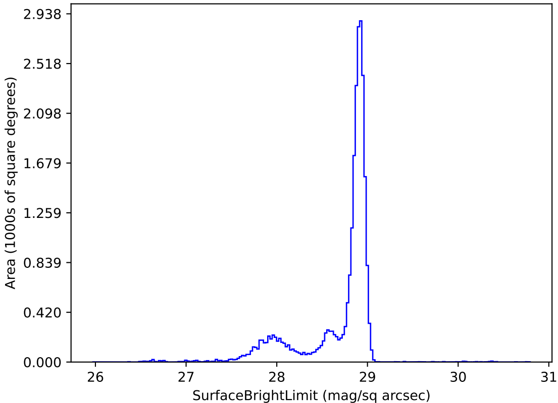
too_10_4v3.4_10yrs u: SurfaceBrightLimit
