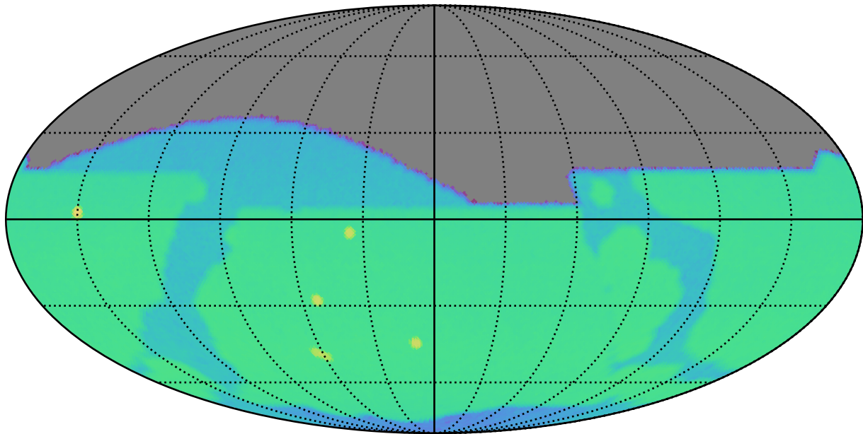
too_10_4v3.4_10yrs r: SurfaceBrightLimit
