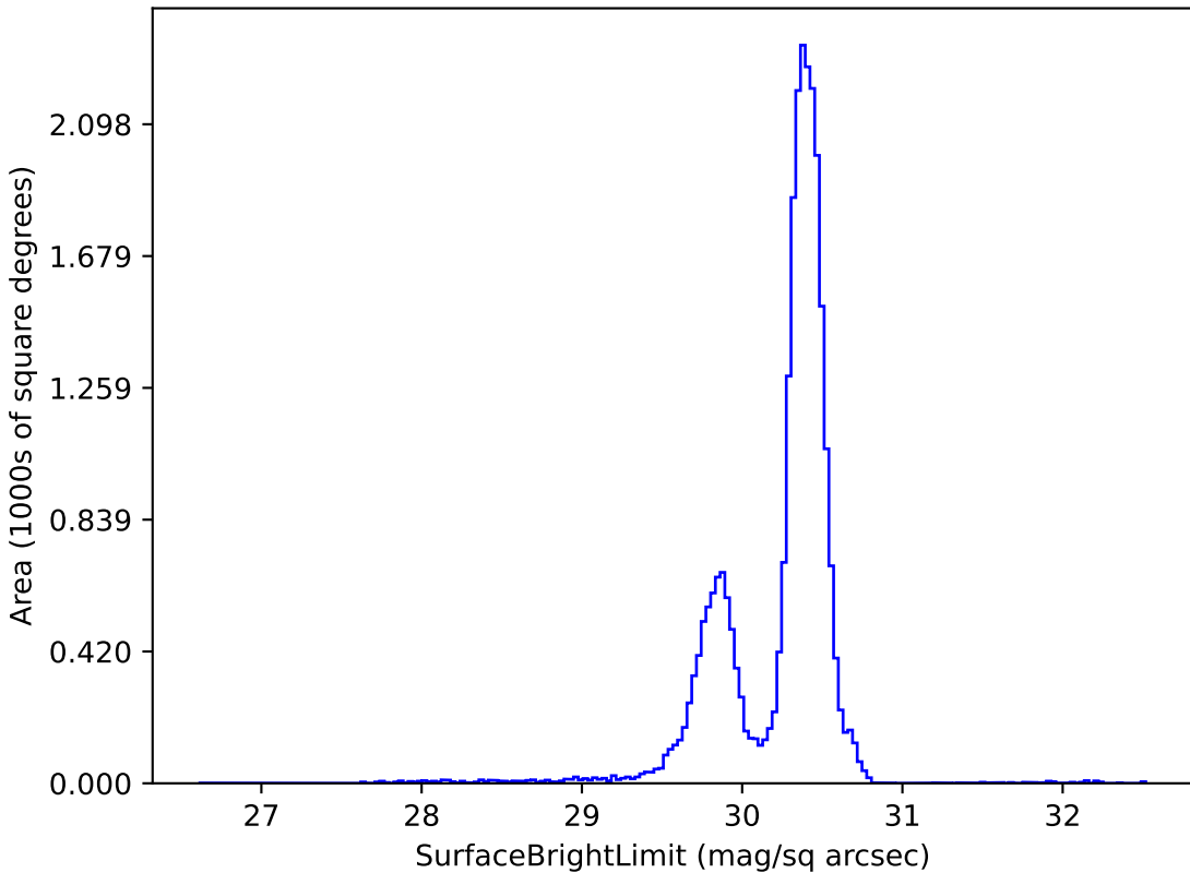
too_10_4v3.4_10yrs g: SurfaceBrightLimit
