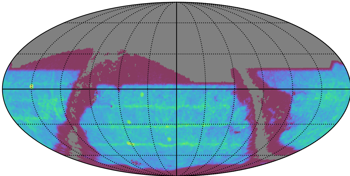
too_10_4v3.4_10yrs : SNSLMetric
