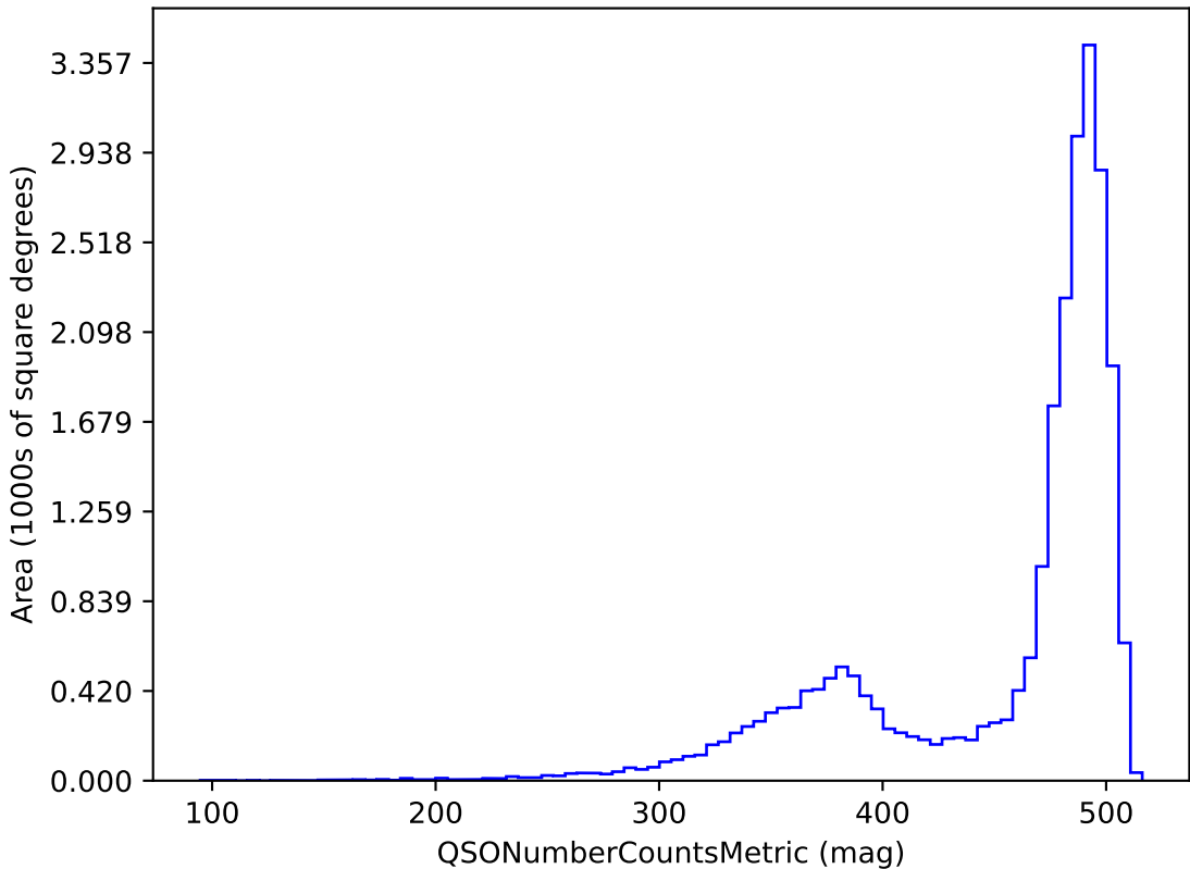
too_10_4v3.4_10yrs z band and non-DD: QSONumberCountsMetric
