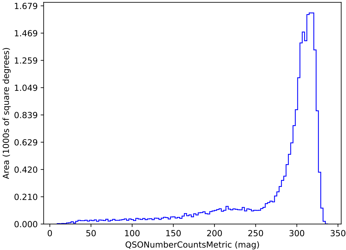
too_10_4v3.4_10yrs u band and non-DD: QSONumberCountsMetric
