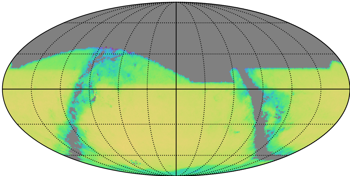
too_10_4v3.4_10yrs r band and non-DD: QSONumberCountsMetric
