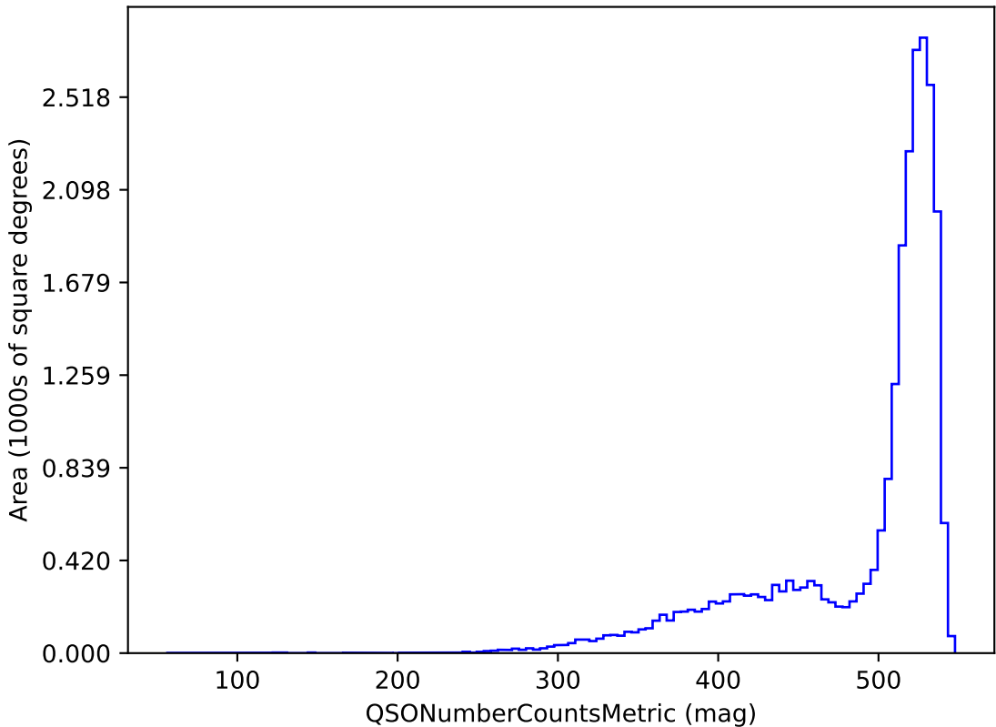
too_10_4v3.4_10yrs r band and non-DD: QSONumberCountsMetric
