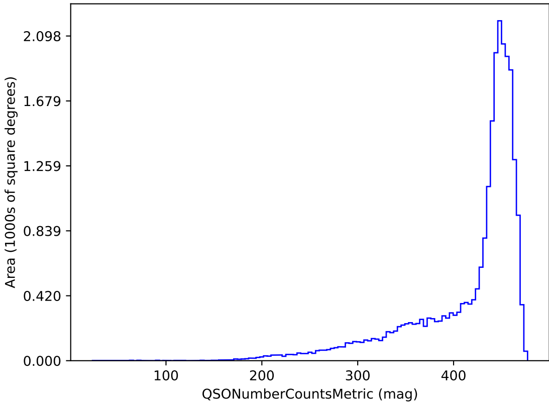
too_10_4v3.4_10yrs g band and non-DD: QSONumberCountsMetric
