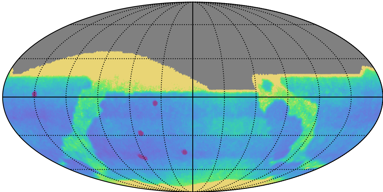
too_10_4v3.4_10yrs : Proper Motion Uncert @ 24.0
