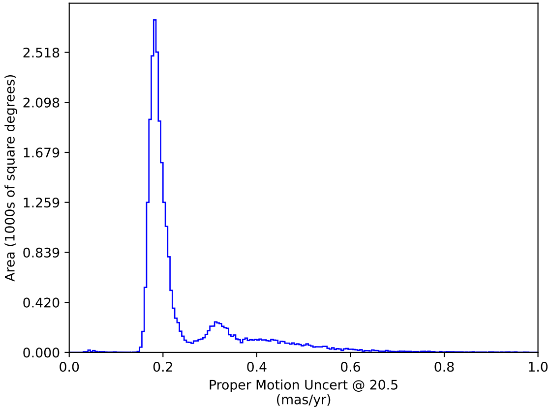
too_10_4v3.4_10yrs : Proper Motion Uncert @ 20.5
