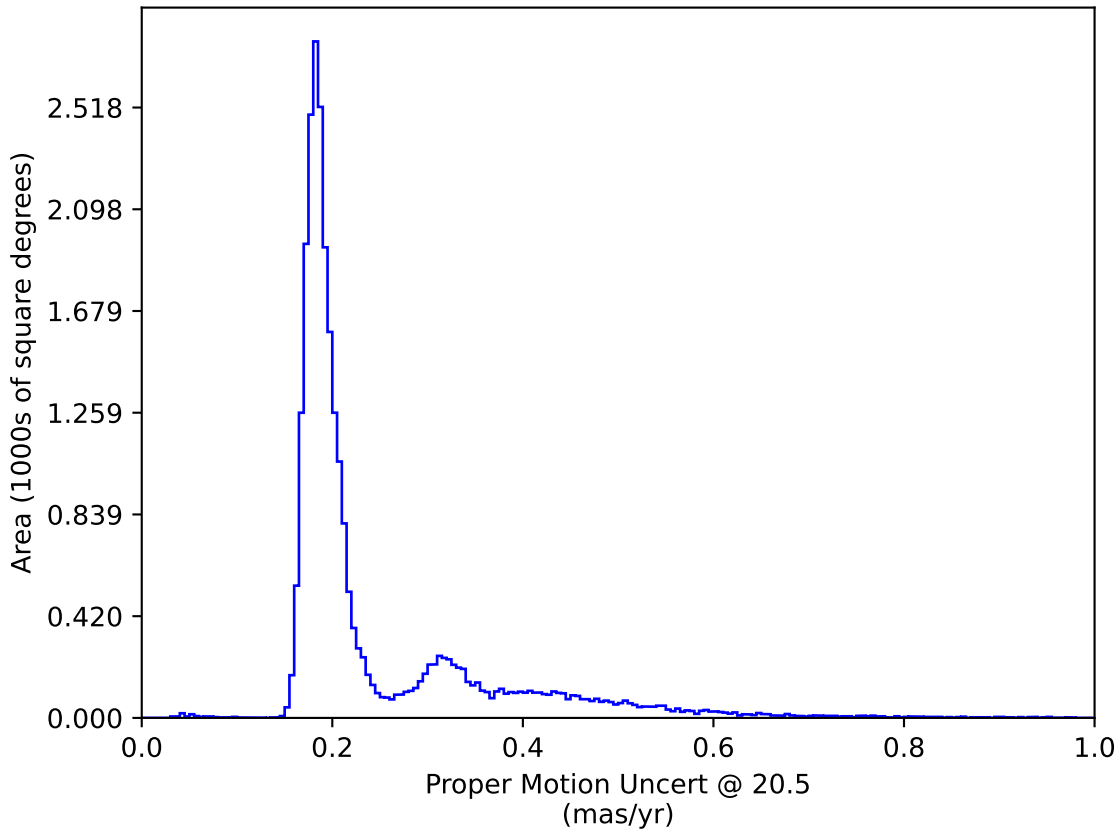
too_10_4v3.4_10yrs : Proper Motion Uncert @ 20.5
