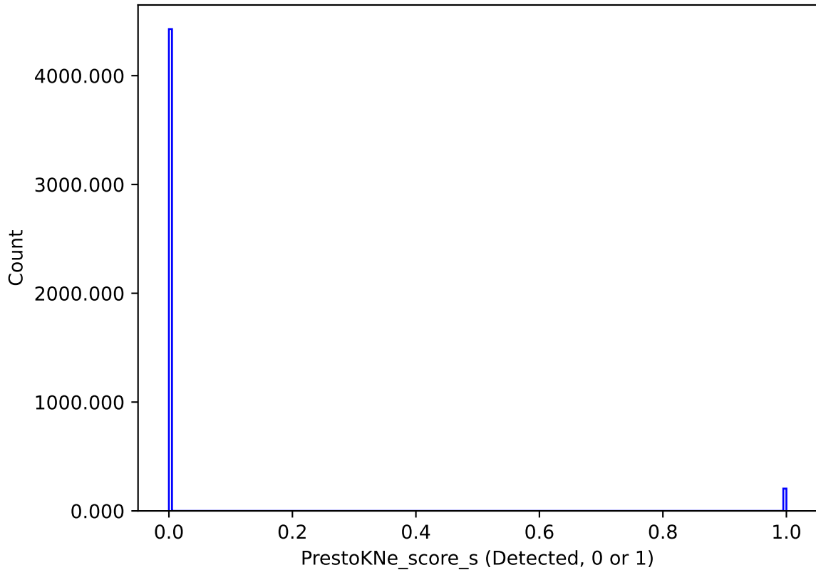
too_10_4v3.4_10yrs : PrestoKNe_score_s
