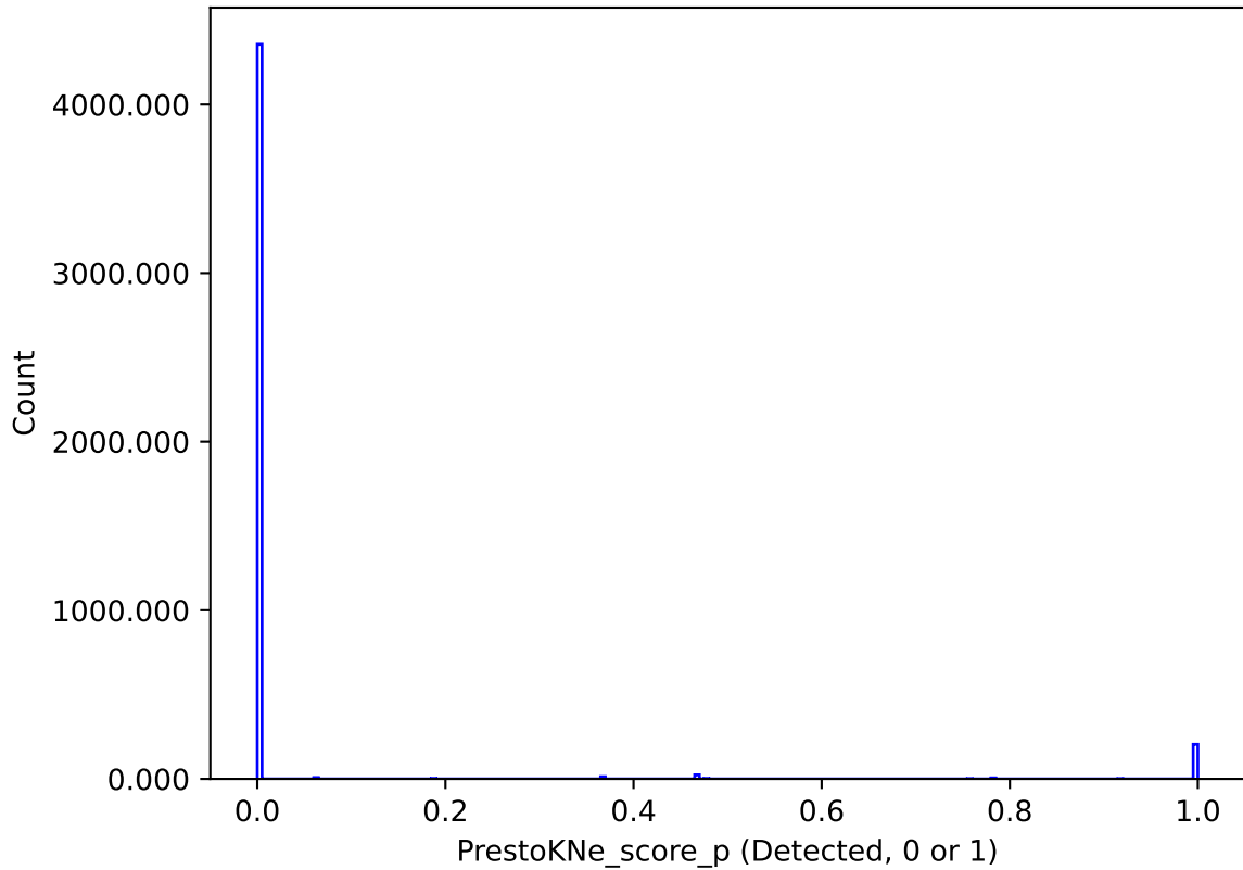
too_10_4v3.4_10yrs : PrestoKNe_score_p
