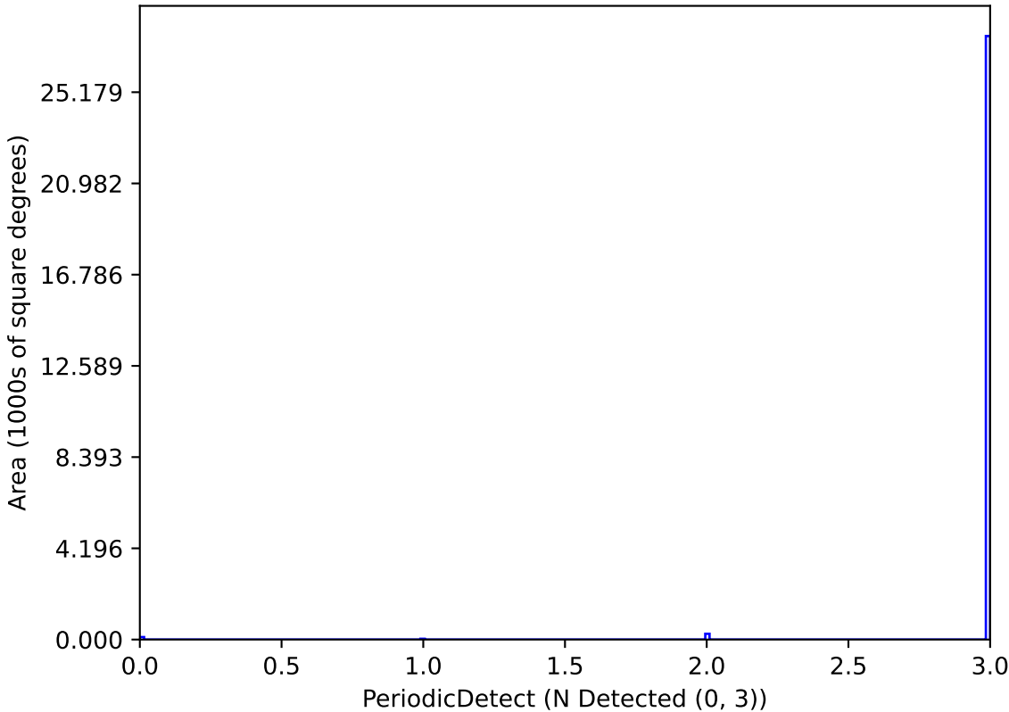
too_10_4v3.4_10yrs P_2.0_Mag_21_Amp_0.05-0.1-1: PeriodicDetect
