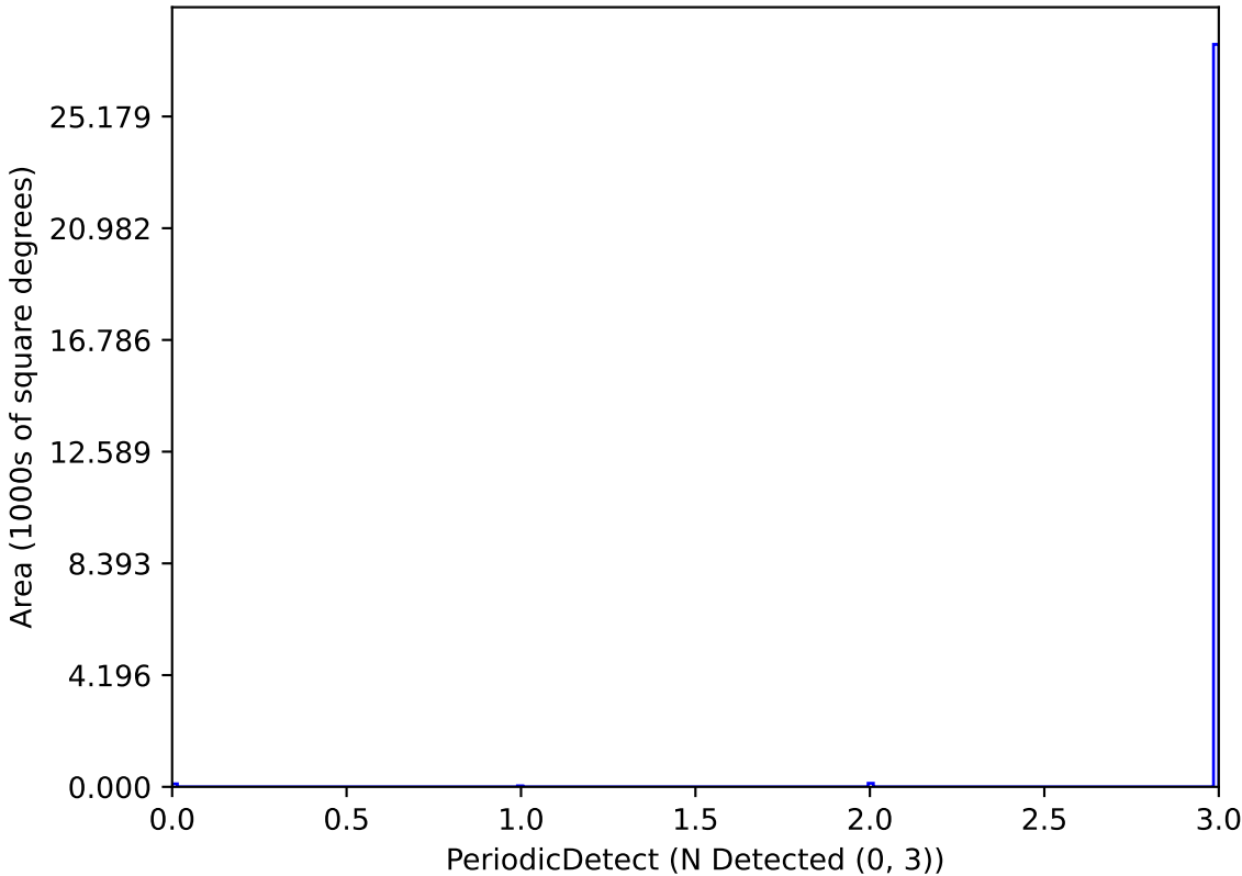
too_10_4v3.4_10yrs P_0.5_Mag_21_Amp_0.05-0.1-1: PeriodicDetect
