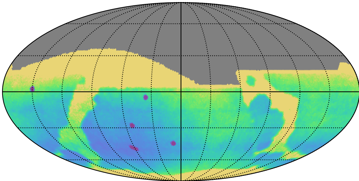
too_10_4v3.4_10yrs : Parallax Uncert @ 24.0
