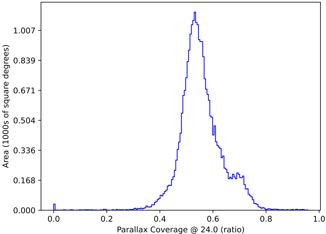
too_10_4v3.4_10yrs : Parallax Coverage @ 24.0
