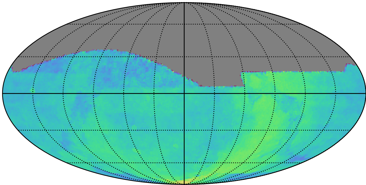
too_10_4v3.4_10yrs : Parallax Coverage @ 22.4
