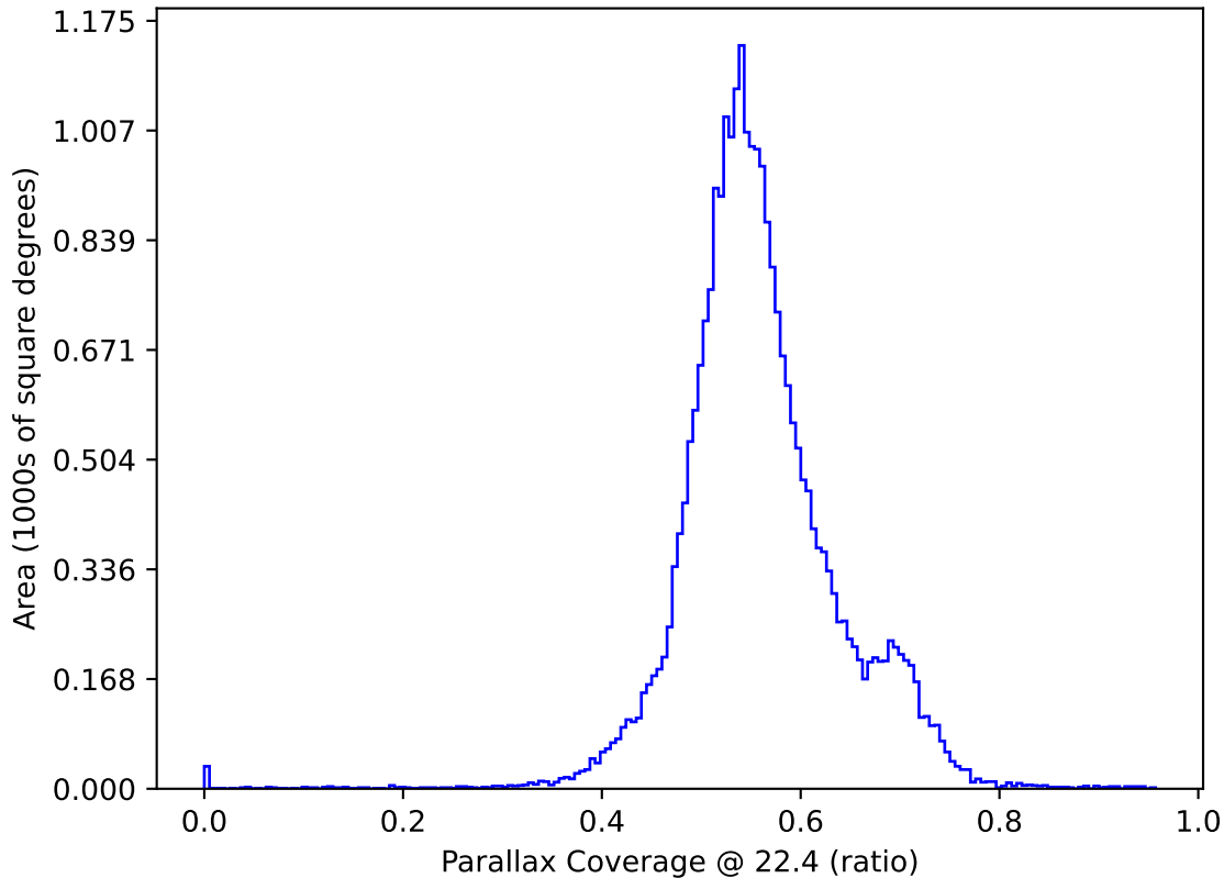
too_10_4v3.4_10yrs : Parallax Coverage @ 22.4
