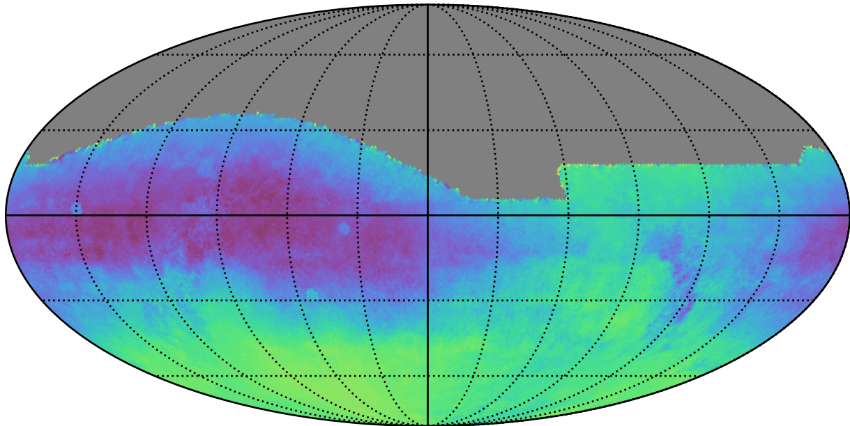
too_10_4v3.4_10yrs : Parallax-DCR degeneracy @ 24.0
