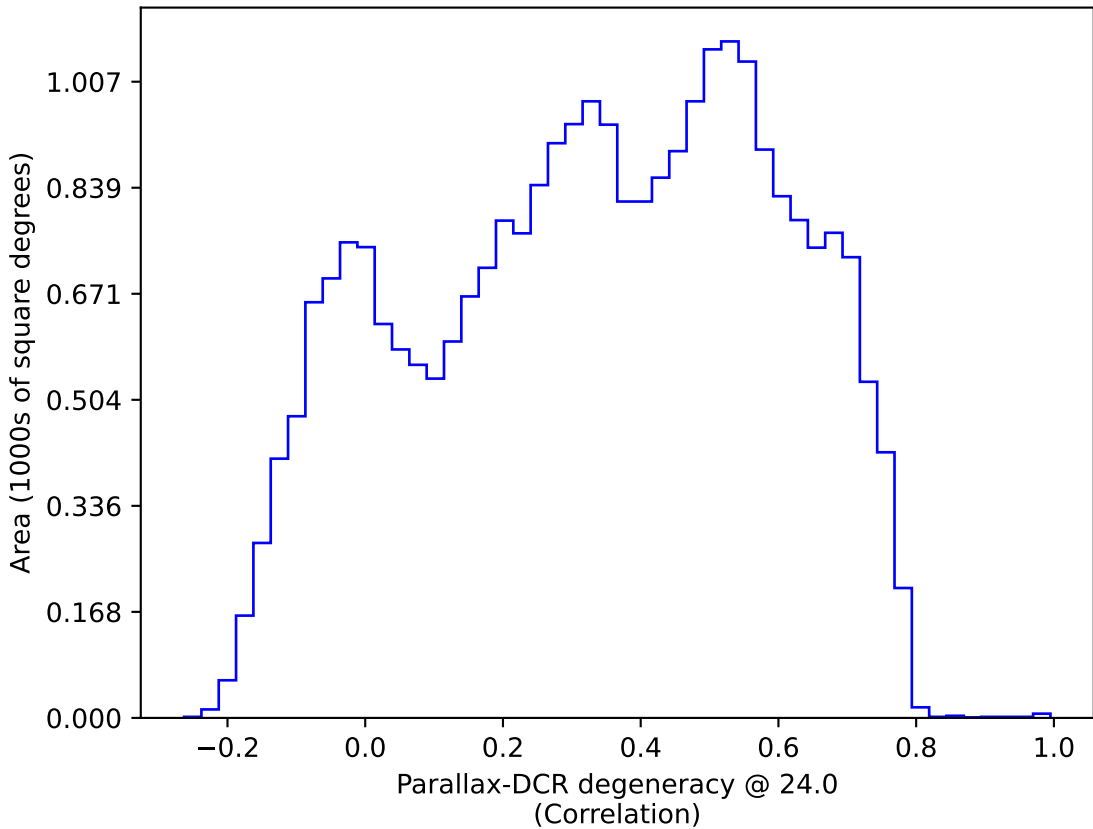
too_10_4v3.4_10yrs : Parallax-DCR degeneracy @ 24.0
