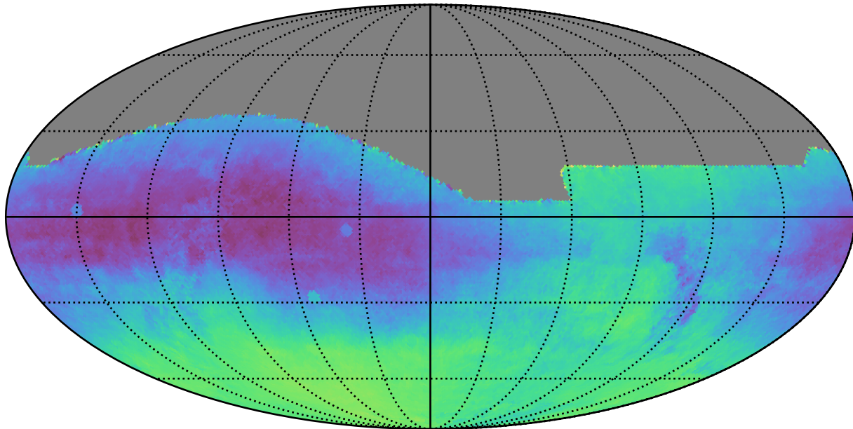
too_10_4v3.4_10yrs : Parallax-DCR degeneracy @ 22.4
