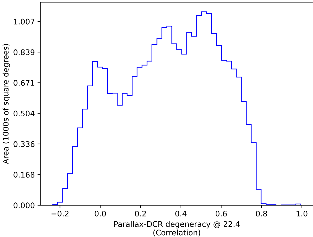
too_10_4v3.4_10yrs : Parallax-DCR degeneracy @ 22.4
