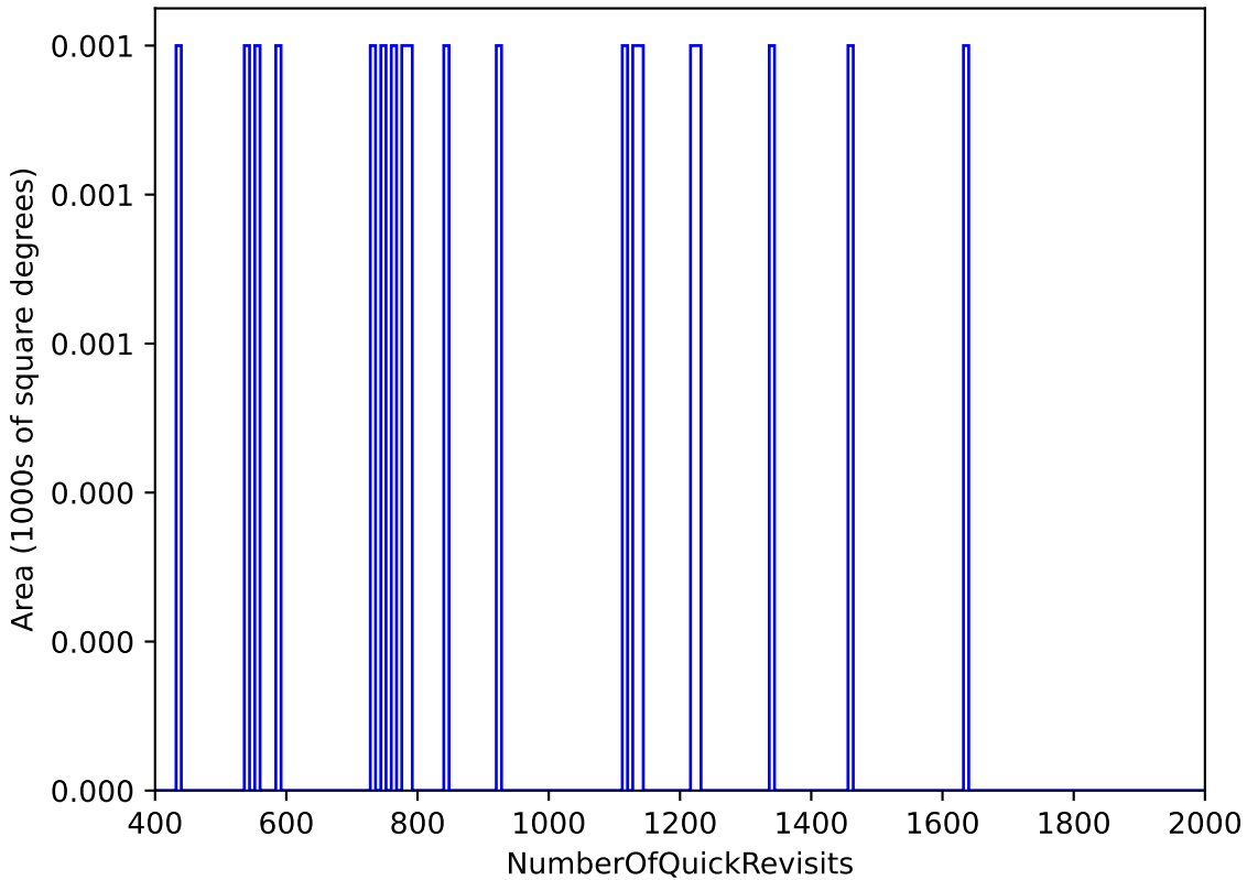
too_10_4v3.4_10yrs : NumberOfQuickRevisits
