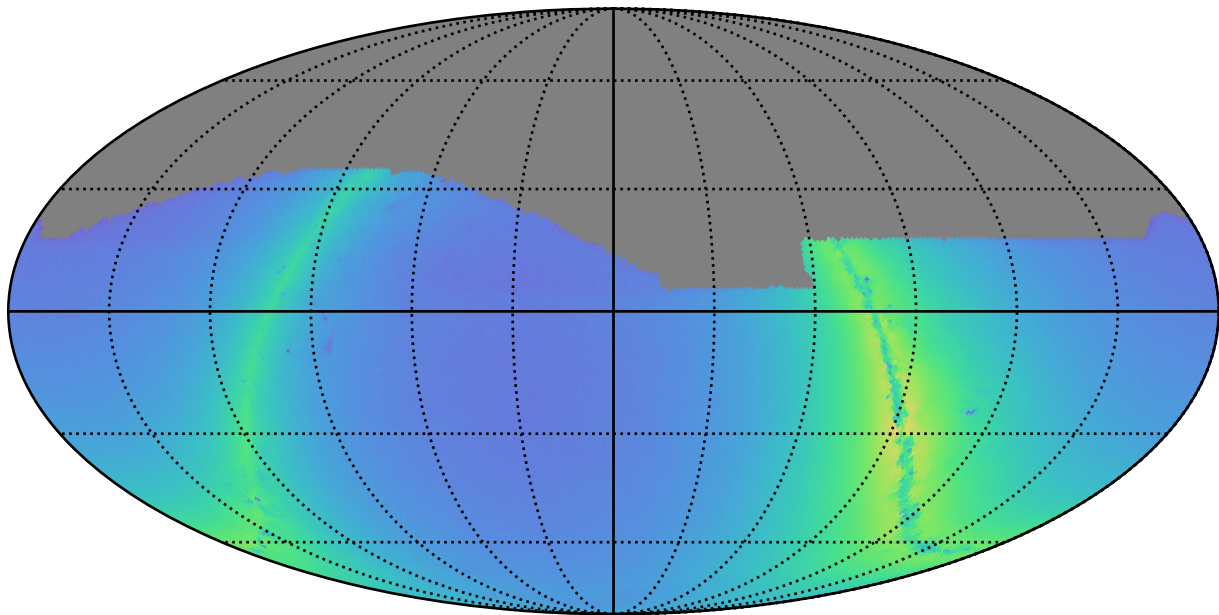
too_10_4v3.4_10yrs z: Nstars_no_crowding
