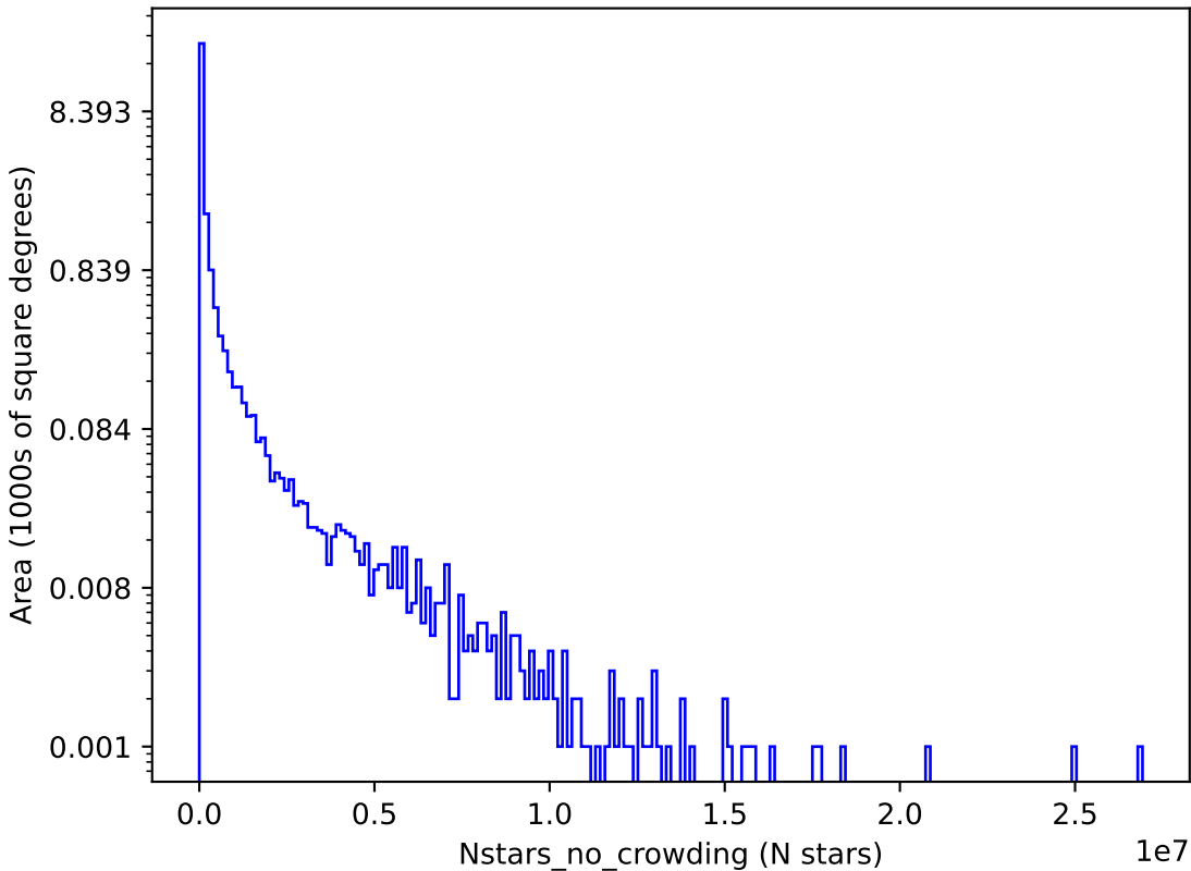
too_10_4v3.4_10yrs z: Nstars_no_crowding
