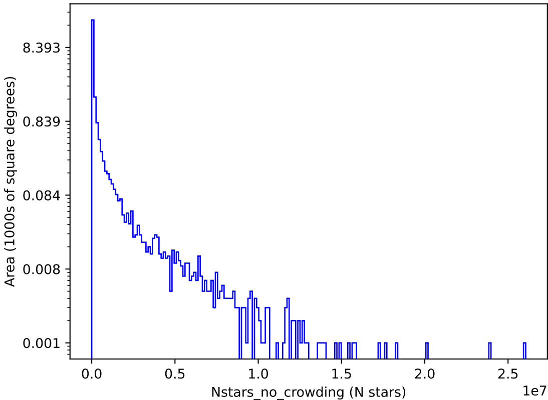
too_10_4v3.4_10yrs y: Nstars_no_crowding
